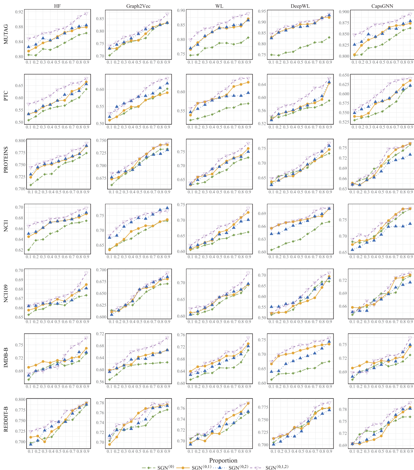
Fig. 10. Average F_1 -Score as functions of the size of the training set (represented by the fraction of samples in the training set), for various feature extraction methods on different datasets, based on SGN (0) , SGN (0,1) , SGN (0,2) and SGN (0,1,2) , respectively.
