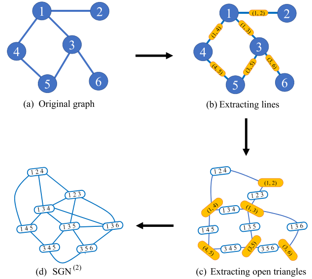
Fig. 3. The process to build SGN^{(2)} from a given network: (a) The original network, (b) extracting lines, (c) building SGN^{(1)} and extracting open triangles as subgraphs, (d) establishing connections among these open triangles to obtain SGN^{(2)} .
